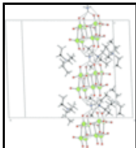
Fig. 2. A partial packing diagram of the title compound with N—H...O hydrogen bonds shown as dashed lines.
